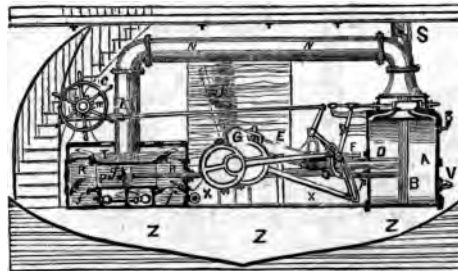
FIG. 186.—Horizontal, Direct-acting Naval Screw-Engine.
